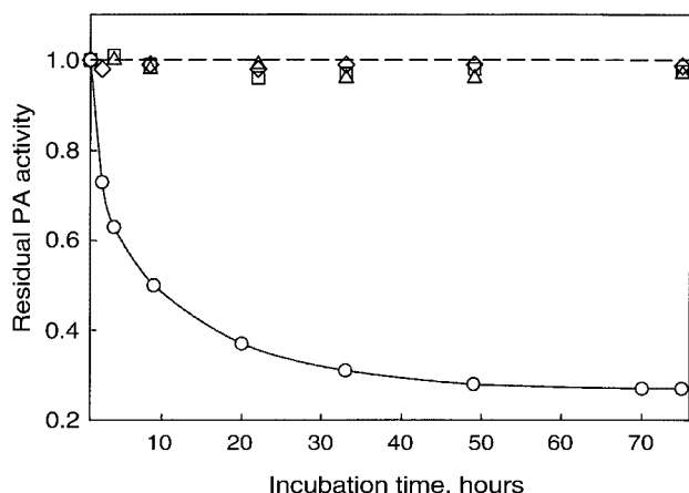
Figure 1. Stability of immobilized penicillin acylase: (○) = immobilized enzyme (the moist preparation), (Δ) = in a mixture with \text{CH}_3\text{COONa} \cdot 3 \text{H}_2\text{O} , (◇) = in a mixture with \text{Na}_2\text{SO}_4 \cdot 10 \text{H}_2\text{O} , (◻) = in a mixture with \text{MgSO}_4 \cdot 7 \text{H}_2\text{O} . In all cases, 30% w/w of salt hydrate was used, a_w = 0.8 . Lines just indicate trends.
