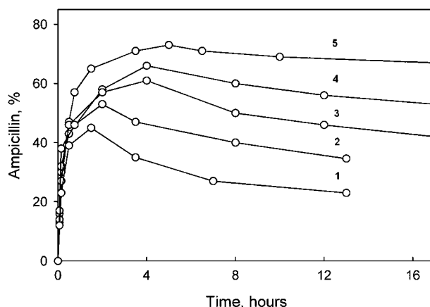
Figure 2. Ampicillin accumulation curves in the penicillin acylase-catalyzed solid-state synthesis. Reaction conditions: (1) = 35, (2) = 30, (3) = 20, (4) = 15, and (5) = 10% w/w of initial water content, 1.4 mmol of 6-APA, 1.4 mmol of D-PGM, 0.5 mmol of \text{Na}_2\text{SO}_4 \cdot 10 \text{H}_2\text{O} , 6 nmol of immobilized PA, a_w = 0.8 .
